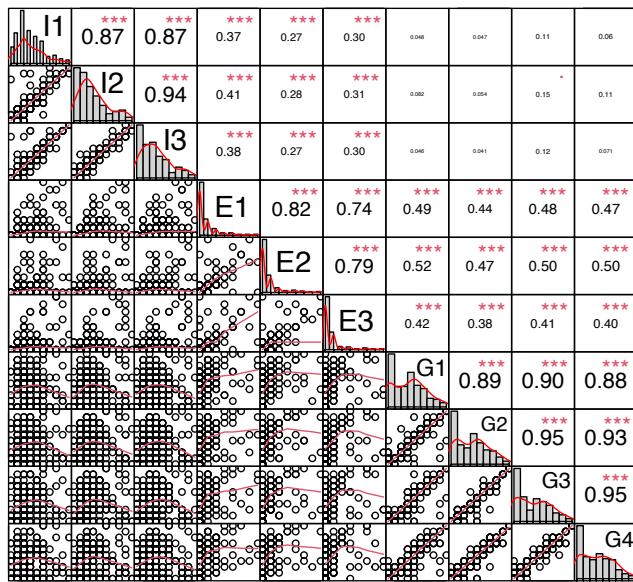
Figure 2: Correlations between items, with corresponding scatter-plots. Three asterisks mark significance at p < 0.001 .
